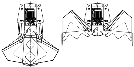
◀ Typ MZG EBS Motor-driven clamshell grab.
